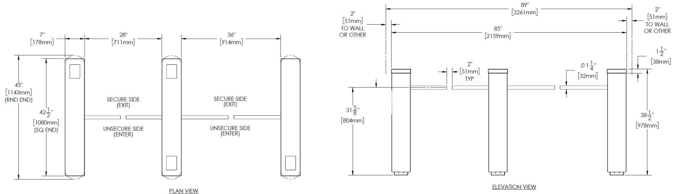
TYPICAL OSAB SA SQ & RND ENDS STANDARD / ADA 2 LANES / 3 PEDS
