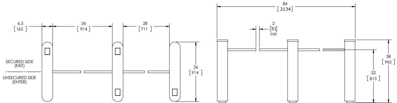
TYPICAL ODAB, ROUND ENDS ONE 28" STANDARD LANE ONE 36" ADA LANE 2 LANE 3 PED
