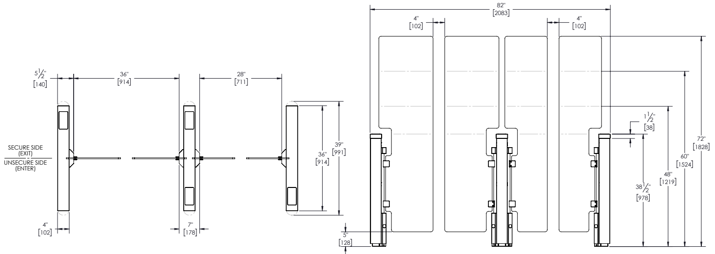
TYPICAL OBSG-TL-C, SQUARE AND ROUNDED ENDS 36" AND 39" ADA LANE AND 28" STANDARD LANE 2 LANE / 3 PED
