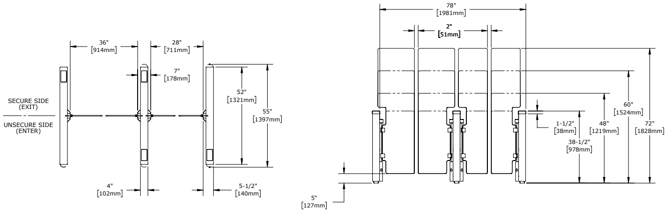
TYPICAL OBSG-TL-CV, SQUARE AND ROUND ENDS 36" ADA LANE AND 28" STANDARD LANE 2 LANE / 3 PED
