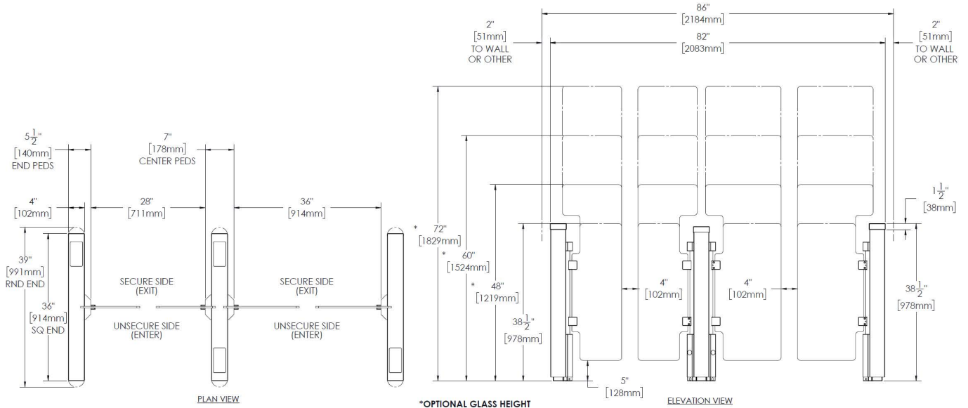
TYPICAL OBSG-TL-C SQ & RND ENDS STANDARD / ADA 2 LANE / 3 PED
