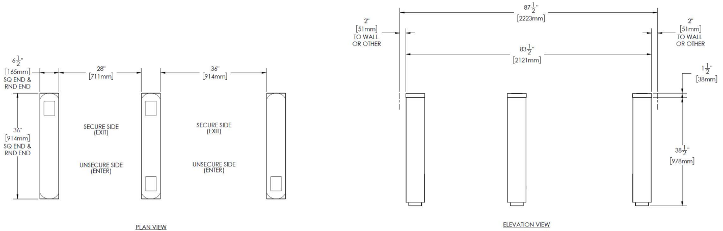
TYPICAL PONB-CV-C SQ & RND ENDS STANDARD / ADA 2 LANES / 3 PEDS
