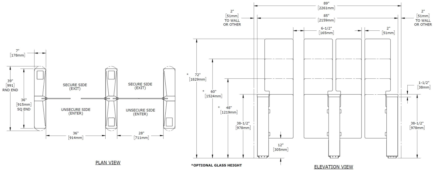
TYPICAL OB SG-HG-C, SQ & RND ENDS ADA / STANDARD 2 LANE / 3 PEDS
