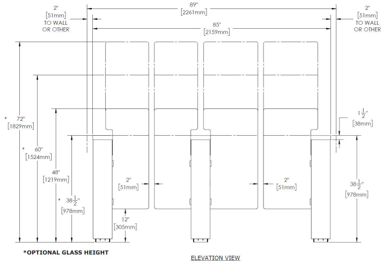
TYPICAL OBSG-HG-CV, SQ & RND ENDS STANDARD / ADA 2 LANE / 3 PED
