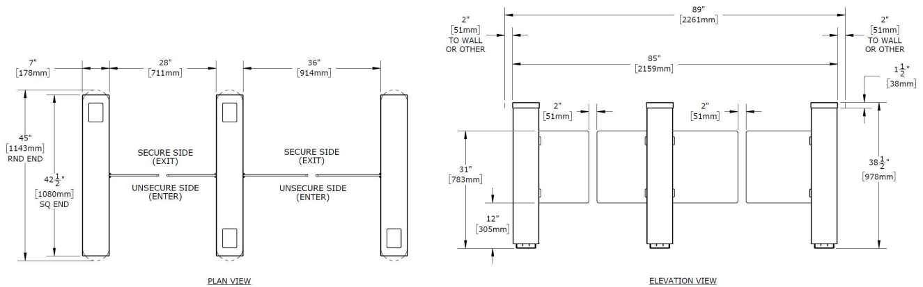
TYPICAL OBSG-LG, SQ & RND ENDS STANDARD / ADA 2 LANES / 3 PEDS
