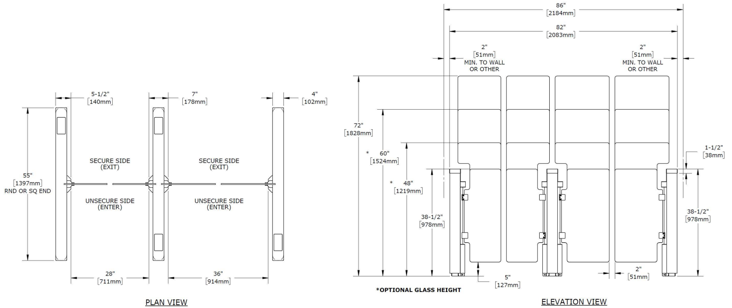
TYPICAL OB SG-TL-CV SQUARE AND ROUND ENDS STANDARD / ADA 2 LANES / 3 PEDS
