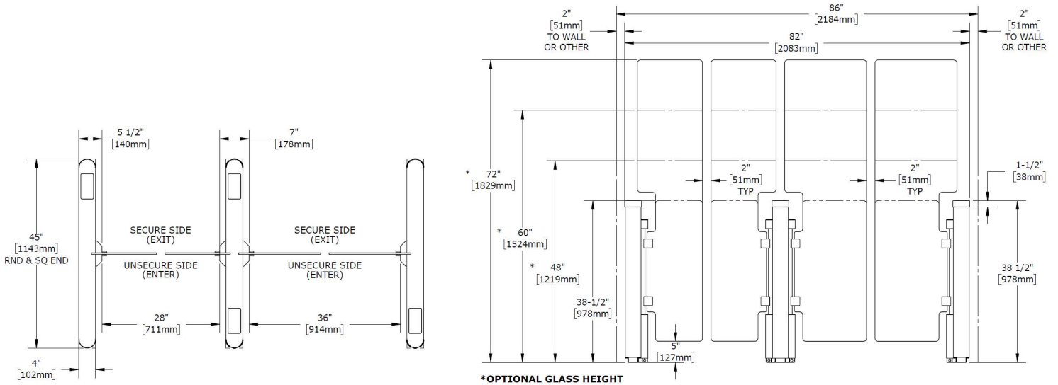
*OPTIONAL GLASS HEIGHT TYPICAL OBSG-TL, SQUARE & ROUND ENDS STD / ADA 2 LANES / 3 PEDS
