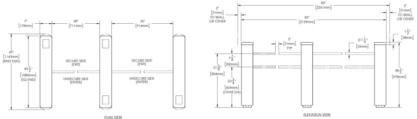
TYPICAL OSAB SA/DA SQ & RND ENDS STANDARD / ADA 2 LANES / 3 PEDS
