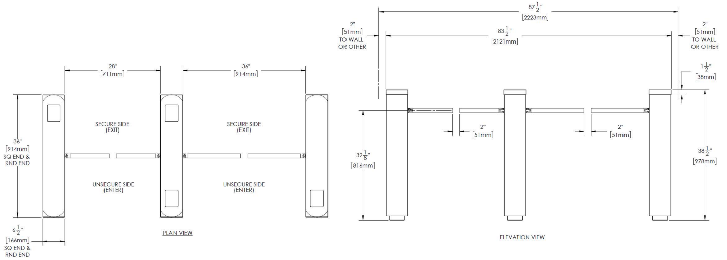
TYPICAL ODAB SQ & RND ENDS STANDARD / ADA 2 LANES / 3 PEDS
